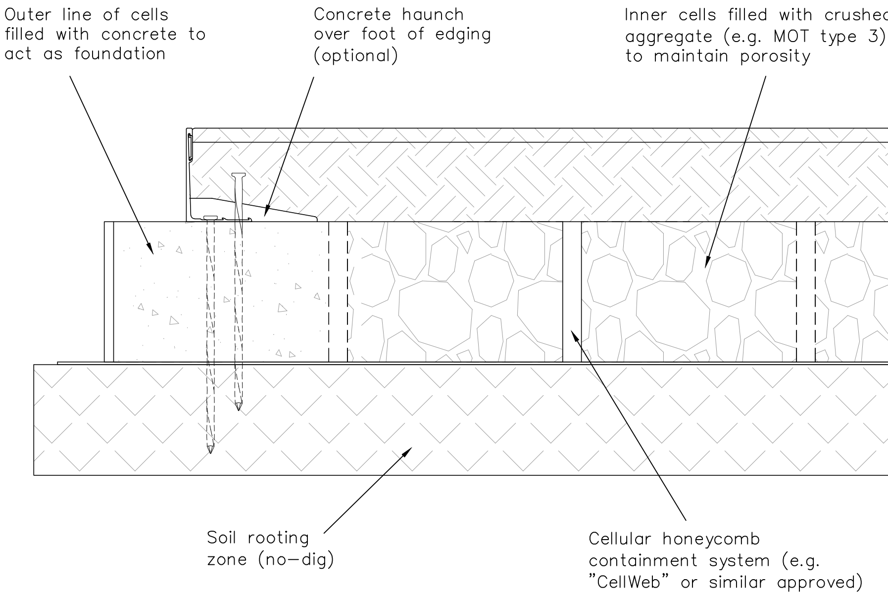
Detail 3 No-Dig
