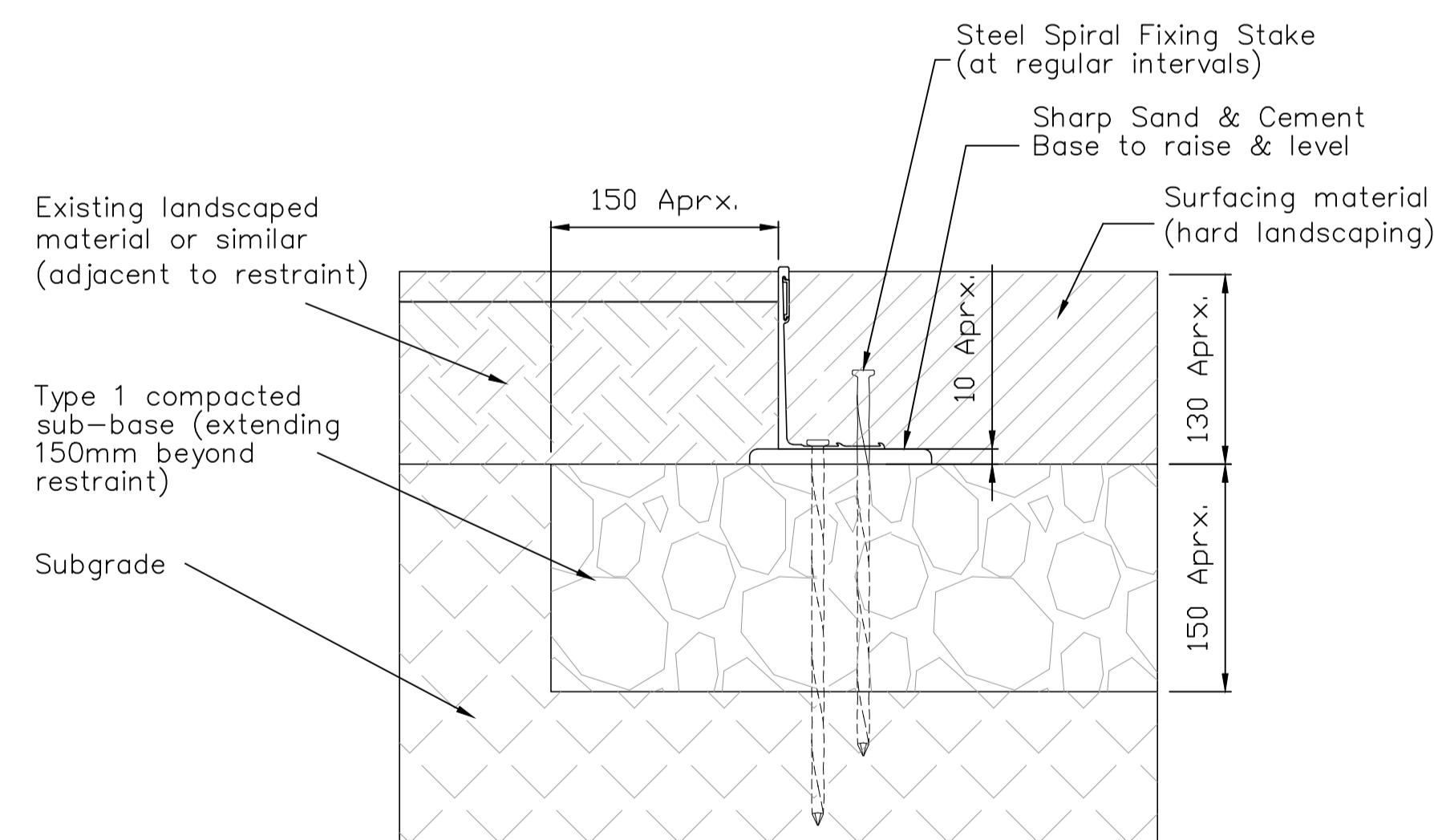
SECTION SCALE 1:4
