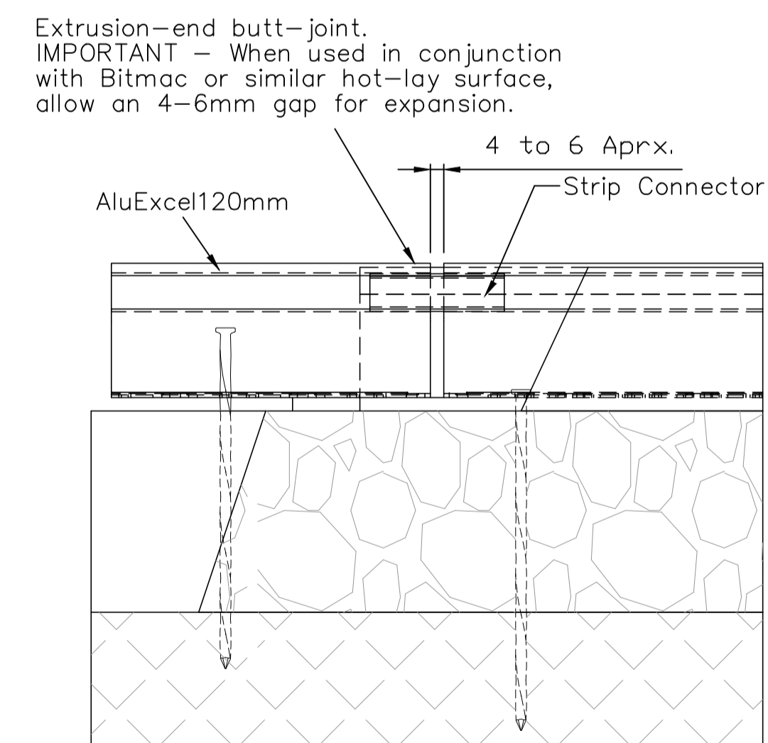
JOINER DETAIL SCALE 1:4
