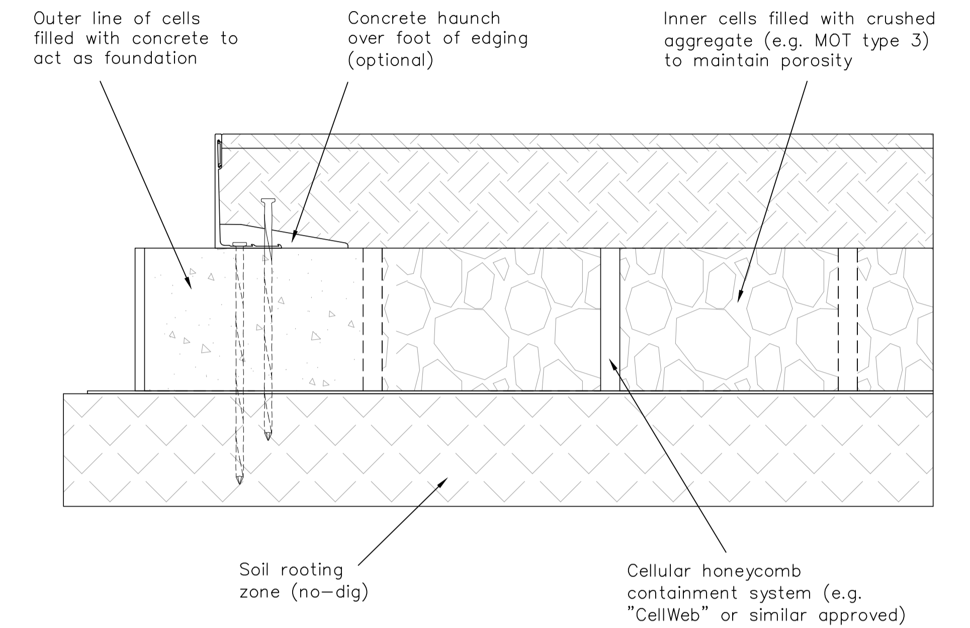
Detail 3 No-Dig
