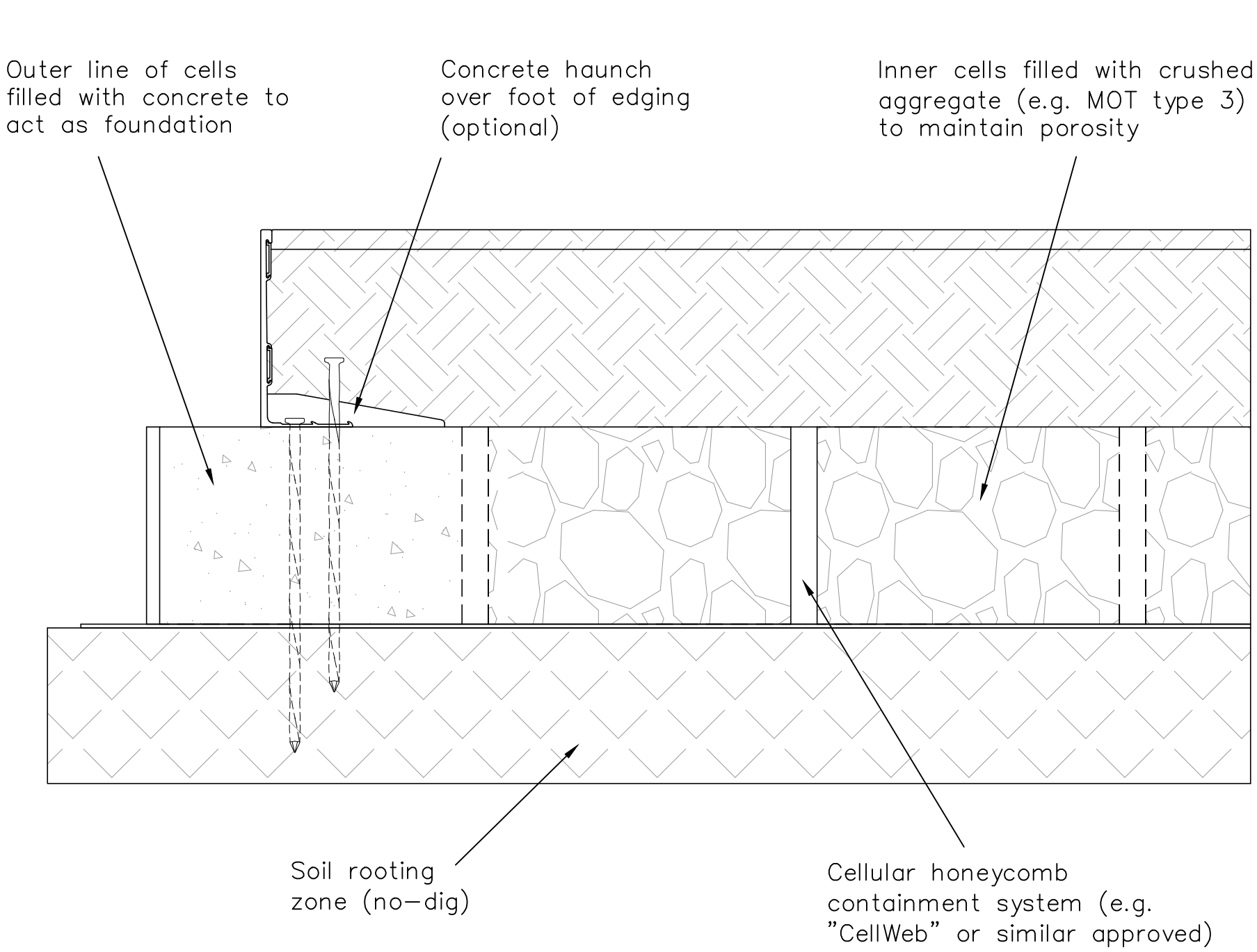
Detail 3 No-Dig
