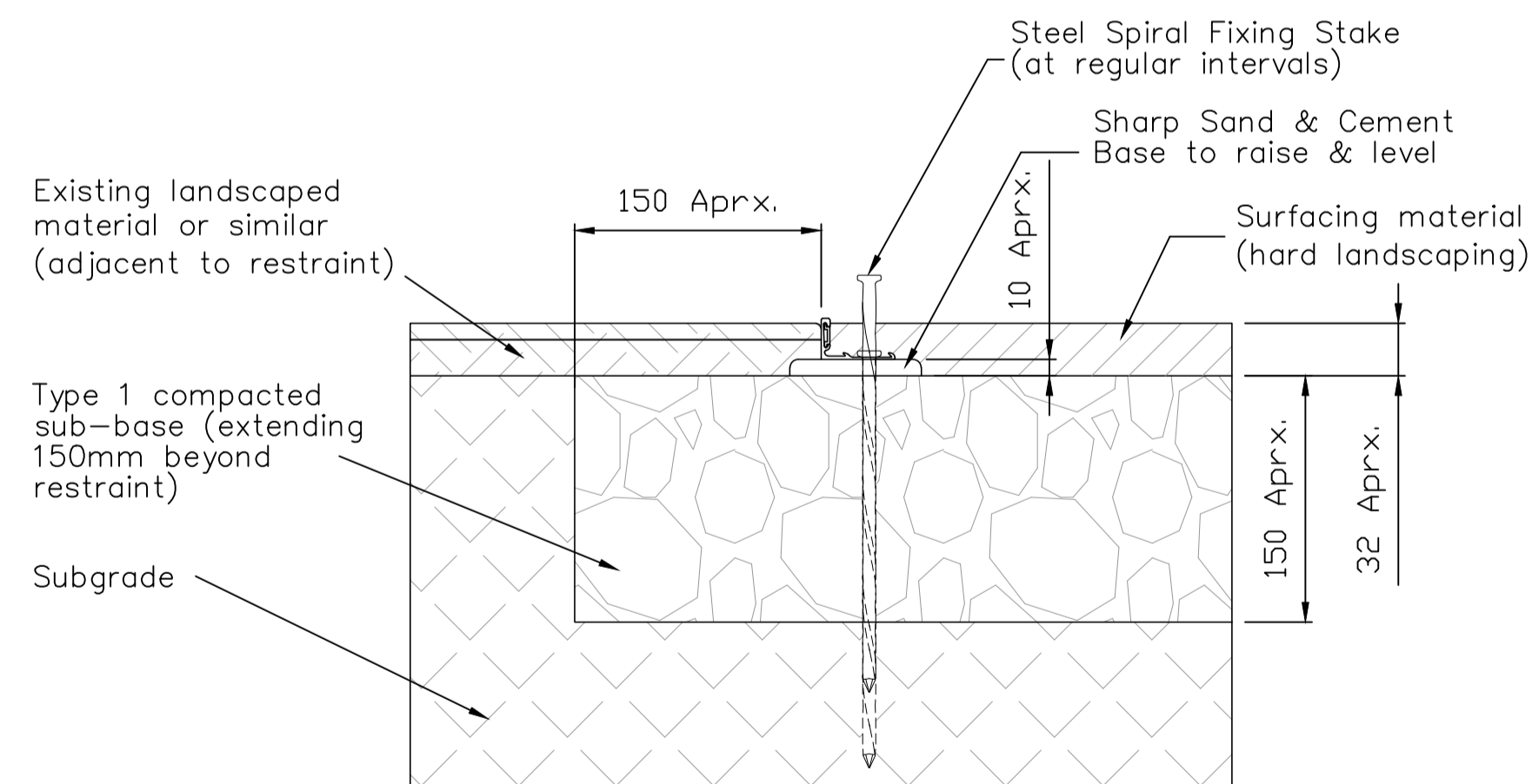
SECTION SCALE 1:4
