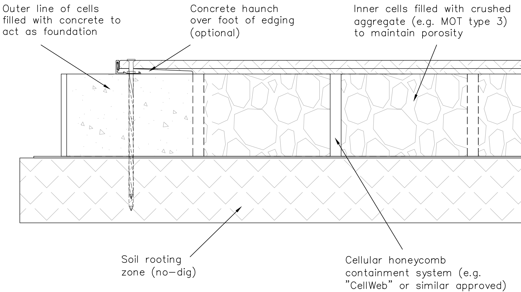
Detail 3 No-Dig
