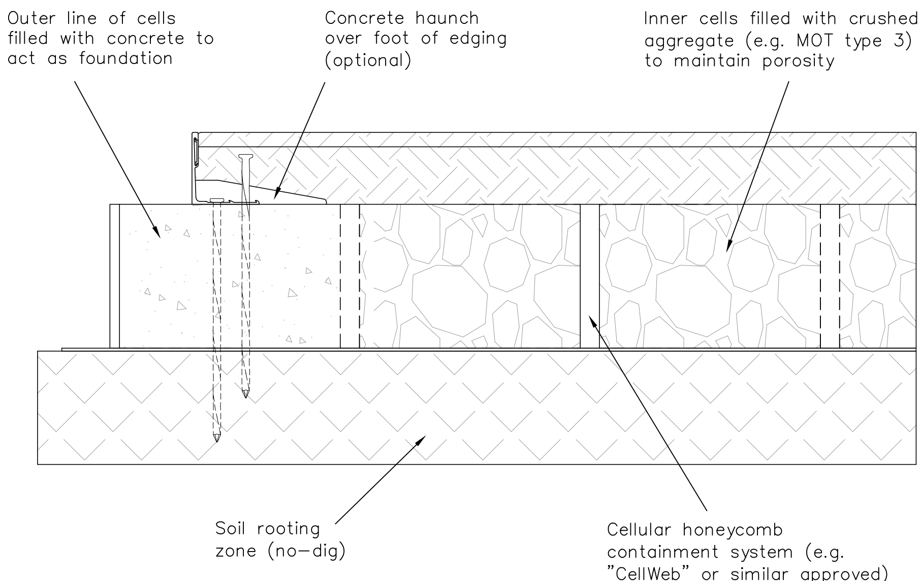
Detail 3 No-Dig
