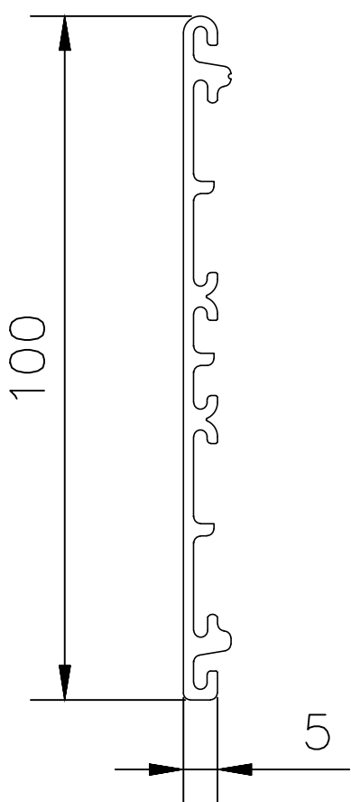
PROFILE SECTION SCALE 1:1
