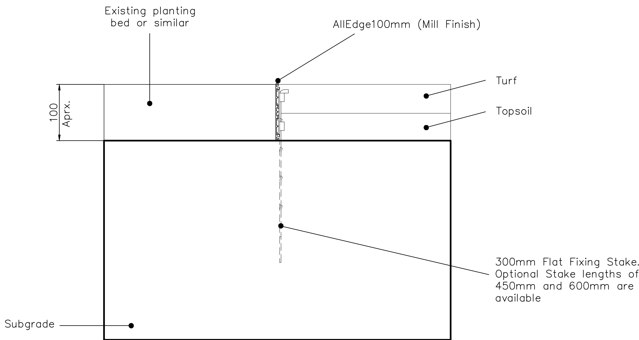
SECTION SCALE 1:4
