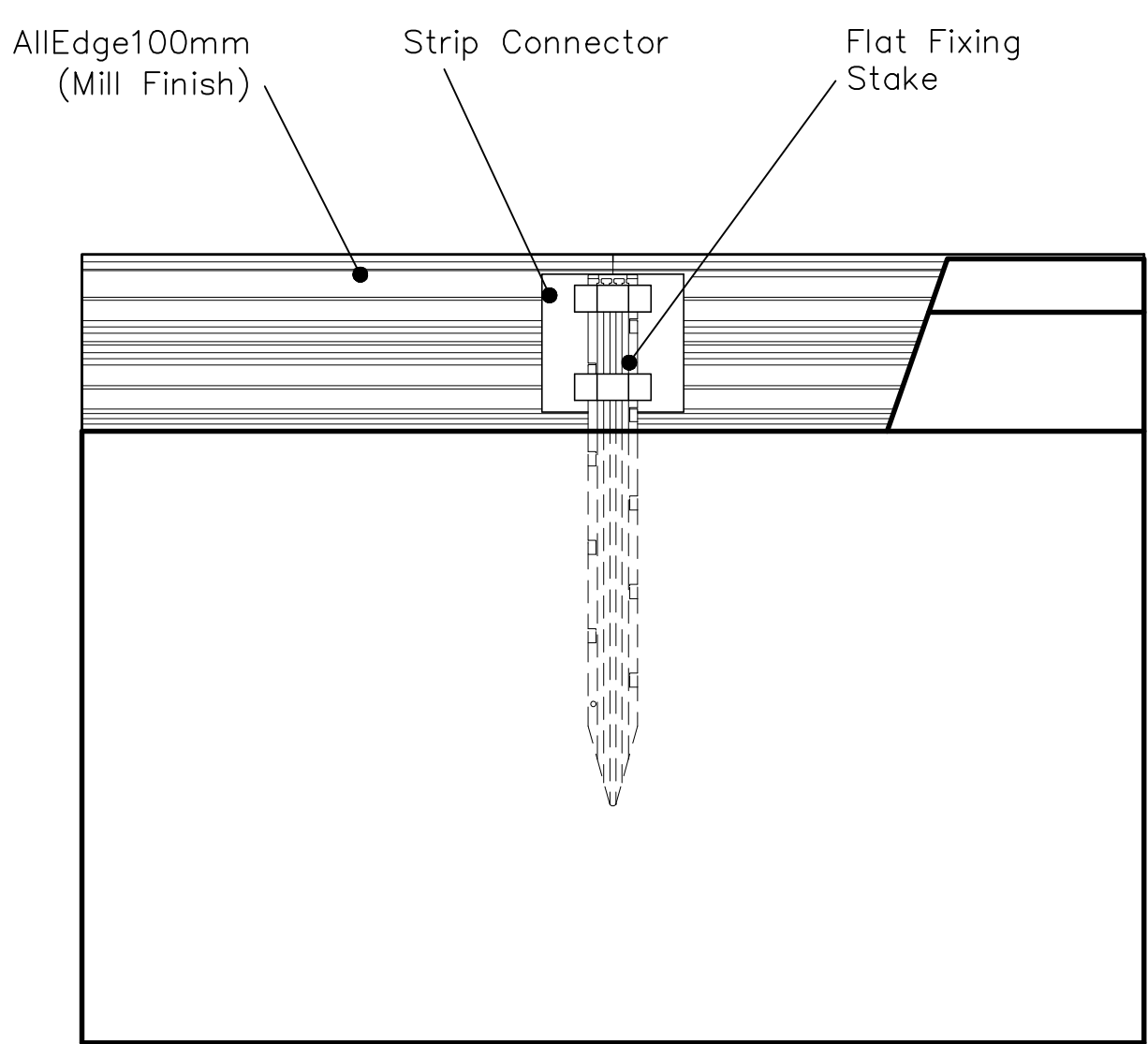
JOINER DETAIL SCALE 1:4
